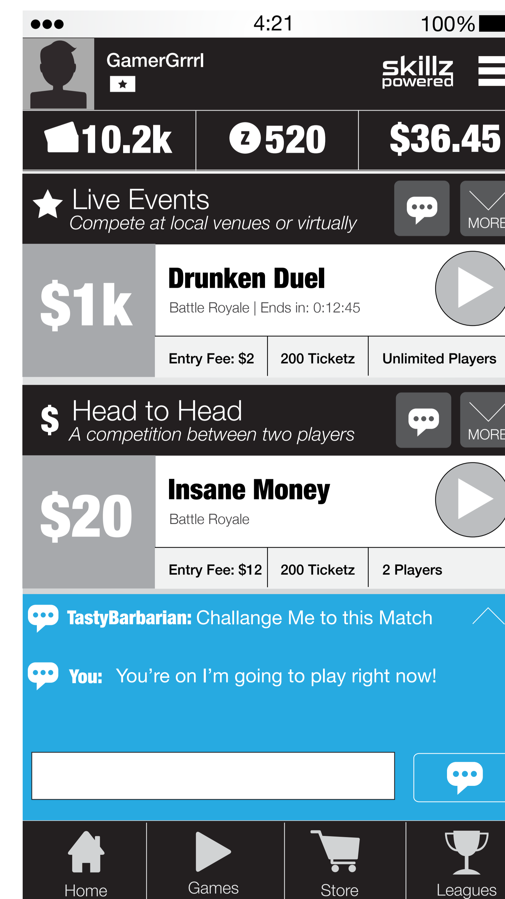
Messages expanded
